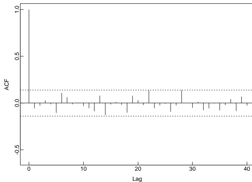
Figure 6-9 The sample ACF of (1 - B + B^2)X_t with \{X_t\} as in Figure 6.7.
