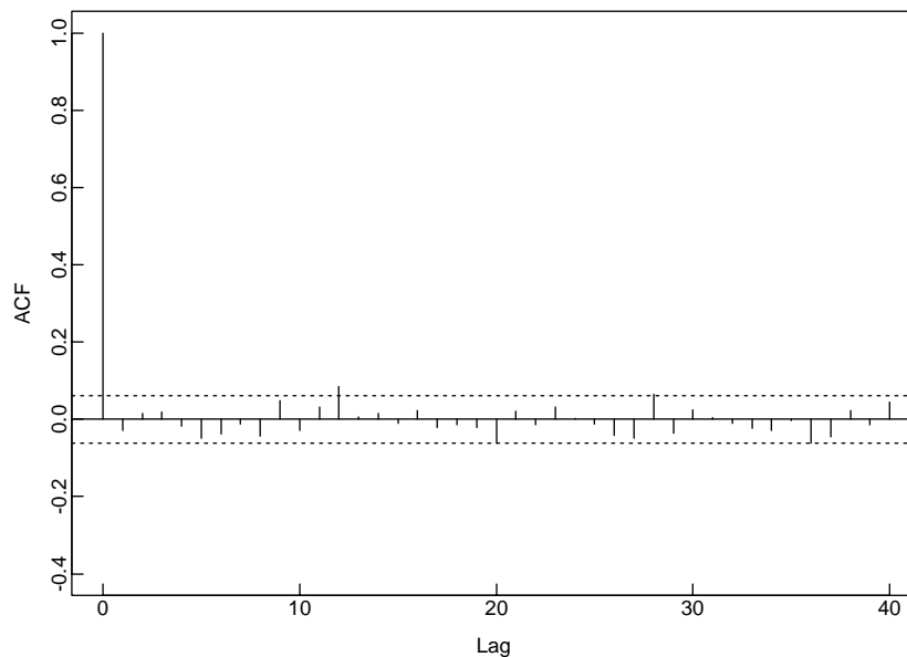
Figure 10-8 The sample autocorrelation function of the series in Figure 10.7.
